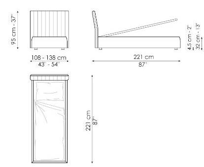
Tonight charme open Width: 108-138cm Depth: 221cm Height: 95cm
