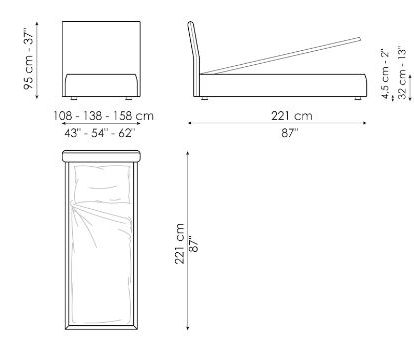
Tonight open Width: 108-138-158cm Depth: 221cm Height: 95cm
