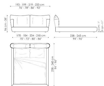
Blend bed plus Width: 193-199-219-233cm Depth: 238-243cm Height: 96cm
