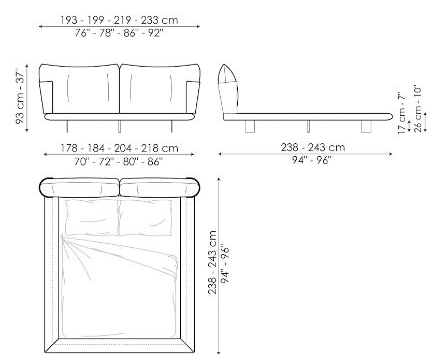
Blend bed Width: 193-199-219-233cm Depth: 238-243cm Height: 96cm
