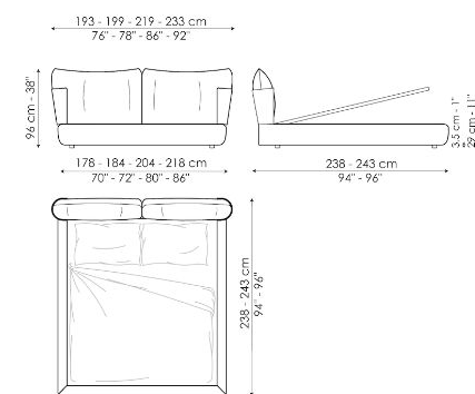
Blend bed open Width: 193-199-219-233cm Depth: 238-243cm Height: 96cm
